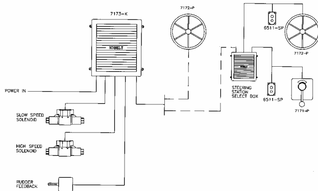
Example of Dual Speed Steering System Arrangement with 7173-K FFU Amplifier
